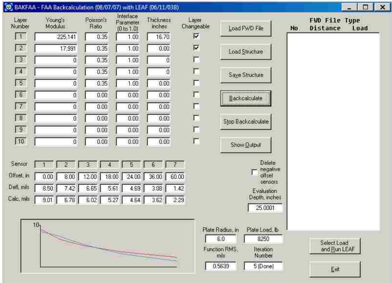
Figure D-6: Example calculated modulus values for step one of the two-step backcalculation process for FWD data.
